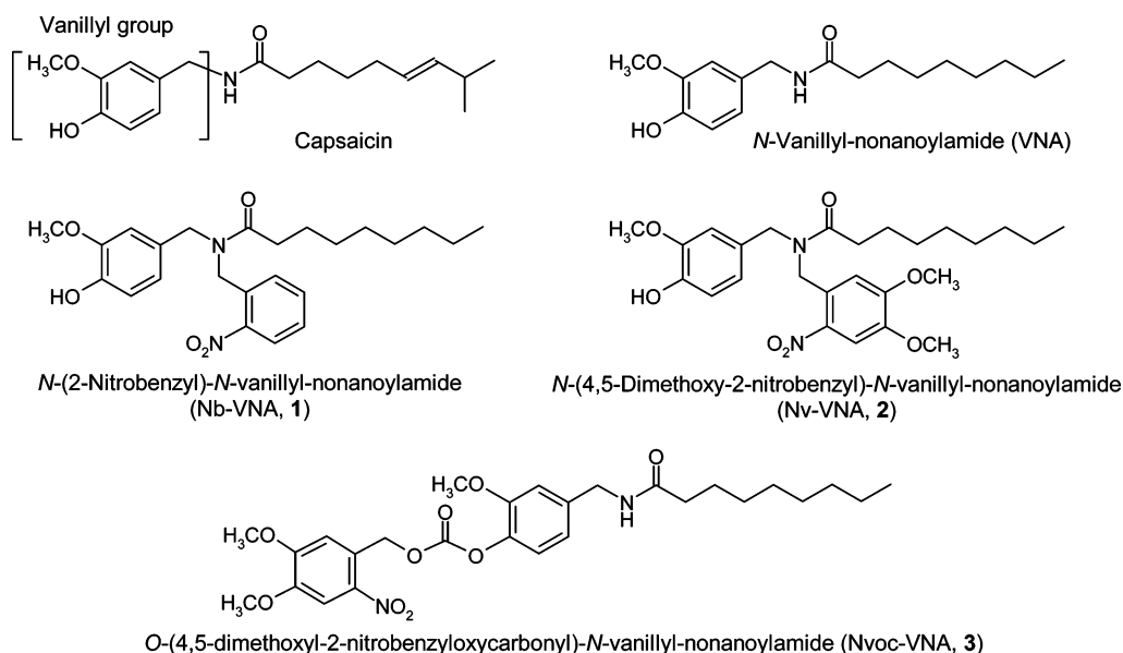
FIGURE 1: Structures of vanilloid molecules. The structures of capsaicin, N -vanillylnonanoylamide (VNA), and the nitrobenzyl- (Nb), nitroveratryl- (Nv), and nitroveratryloxycarbonyl- (Nvoc) caged versions of VNA are shown.
