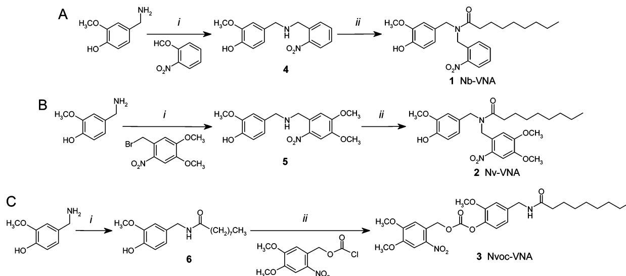
FIGURE 2: Synthetic schemes for the caged vanilloids, Nb-VNA, Nv-VNA, and Nvoc-VNA. Reaction conditions: (A) (i) \text{Na}(\text{CH}_3\text{CO}_2)_3\text{-BH} , \text{NaOAc} , 1,2-dichloroethane; (ii) \text{K}_2\text{CO}_3 , \text{Et}_3\text{N} , dichloromethane. (B) (i) 1,2,2,6,6-pentamethylpiperidine, DMF/acetonitrile; (ii) \text{K}_2\text{CO}_3 , \text{Et}_3\text{N} , dichloromethane. (C) (i) n -Nonanoic acid N -hydroxysuccinimidyl ester, \text{Et}_3\text{N} , \text{EtOAc} /DMF; (ii) \text{Et}_3\text{N} , dichloromethane.
