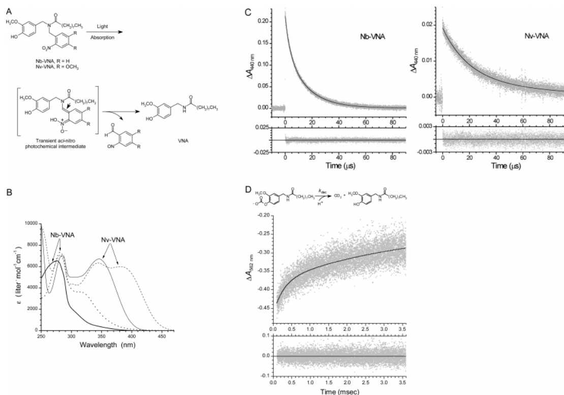
FIGURE 3: Spectroscopic characterization of the photorelease of N -vanillylnonanoylamide (VNA) from caged VNA. (A) Photolysis of caged VNA. Light absorption by caged VNA generates the short-lived aci -nitro intermediate, which decomposes into the spent cage (a 2-nitrosobenzaldehyde) and VNA. The aci -nitro intermediate can exist in two geometric isomeric forms: the configuration around the double bond marked by the arrowhead can be either E or Z . For the Nb cage, R = H; for the Nv cage, R = OCH 3 . (B) UV–visible absorption spectra of caged VNAs. Spectra of Nb-VNA acquired before (thick solid line) and after (dotted line) photolysis. Spectra of Nv-VNA acquired before (thin solid line) and after (dashed line) photolysis. Photolysis was for 30 s with 375 mW of the UV emission from an argon ion laser. (C) Transient absorbance spectral changes of Nb-VNA and Nv-VNA following laser flash photolysis. The absorbance at 440 nm of a solution of Nb-VNA or Nv-VNA in acetonitrile was monitored. At time zero, an 8.6-ns pulse of 355-nm light was delivered to the sample. In each case, in the larger panel, gray points are experimental data and the solid black curve is the nonlinear least-squares double-exponential fit to the data; the residuals of the least-squares fit are shown in the smaller lower panel. For Nb-VNA, the two exponential components have time constants \tau_1 = 3.47 \pm 0.05 \mu\text{s} and \tau_2 = 15.3 \pm 0.1 \mu\text{s} , and account for 34% and 66% of the total transient absorbance change, respectively. For Nv-VNA, the two exponential components have time constants \tau_1 = 19.3 \pm 2.1 \mu\text{s} and \tau_2 = 71 \pm 58 \mu\text{s} , and account for 71% and 29% of the total transient absorbance change, respectively. Data shown for Nb-VNA are the average of 5 replicate measurements; data shown for Nv-VNA are the average of 25 replicate measurements. Pulse energies were \sim 200 mJ and \sim 50 mJ for Nb-VNA and Nv-VNA, respectively. (D) Kinetics of decarboxylation of VNA-carbonate monitored indirectly with the pH indicator Phenol Red. Generated by photolysis of Nvoc-VNA, VNA-carbonate, the monocarbonate ester of VNA, undergoes decarboxylation, with proton uptake, to yield carbon dioxide and free VNA. The unimolecular rate constant for decarboxylation is k_{\text{dec}} . To monitor decarboxylation kinetics, the absorbance of a solution of Nvoc-VNA (525 \mu\text{M} ) in methanol–water (8:2) containing 40 \mu\text{M} Phenol Red indicator was monitored at 562 nm. At time zero, an 8.6-ns, 30-mJ pulse of 355-nm light was delivered to the sample. In the upper panel, gray points are experimental data (average of a total of 20 traces) showing the rising phase of the Phenol Red absorbance signal, and the solid black curve is the nonlinear least-squares double-exponential fit to the data. The two exponential components have time constants \tau_{\text{slow}} = 3.50 \pm 1.29 ms and \tau_{\text{fast}} = 270 \pm 40 \mu\text{s} , and correspond to 37% and 63% of the absorbance increase, respectively. The residuals of the least-squares fit are shown in the lower panel. Before the experiment, the sample was adjusted to pH 8.1 and purged with, and sealed under, argon gas.
