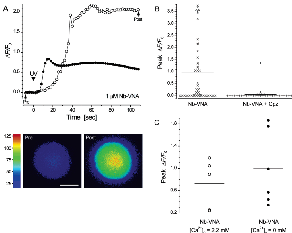
FIGURE 4: [Ca^{2+}]_i signals in DRG neurons in response to in situ UV photolysis of Nb-VNA. (A) In situ photolysis of Nb-VNA evokes robust [Ca^{2+}]_i rises in DRG neurons. Fluorescence traces acquired in two separate experiments from single isolated DRG neurons that had been loaded with the fluorescent Ca^{2+} indicator, fluo-3. Each neuron was superfused for 5 min with Locke solution containing 1 \mu M Nb-VNA. Thereafter, a 20-ms UV pulse (arrowhead marked "UV") evoked a marked rise in [Ca^{2+}]_i , as reflected by the increase in fluo-3 fluorescence. The traces show that both the maximal amplitude and the rise time of the vanilloid-evoked Ca^{2+} response can vary among cells. Representative pre- and postphotolysis confocal fluorescence images of the neuron, corresponding to points in the trace marked by arrows, are shown below the graph. Fluorescence intensity in the images is encoded in pseudocolor. Scale bar = 10 \mu m. In all experiments shown in Figure 4, UV exposure at the specimen was 14 \mu J/ \mu m 2 . (B) Capsazepine, a vanilloid receptor antagonist, blocks the [Ca^{2+}]_i rise in DRG neurons evoked by photolysis of Nb-VNA. In the absence of 5 \mu M capsazepine (Cpz), UV photorelease of VNA from Nb-VNA evoked detectable [Ca^{2+}]_i rises in the majority of DRG neurons (30 of 46). In the presence of 5 \mu M capsazepine, only 1 of 39 DRG neurons showed a sizable rise in [Ca^{2+}]_i . The data were binned in increments of 0.05 on the \Delta F/F_0 scale. Solid horizontal lines indicate the mean peak \Delta F/F_0 for each distribution: without Cpz, 0.99 \pm 0.19 ( n = 46 ); with Cpz, 0.055 \pm 0.035 ( n = 39 ). (C) Photoreleased vanilloid can elevate [Ca^{2+}]_i in the absence of extracellular Ca^{2+} . In normal Locke solution ( [Ca^{2+}]_o = 2.2 mM), UV photorelease of VNA evoked a [Ca^{2+}]_i rise in 5 out of 11 DRG neurons. In Ca^{2+} -free Locke solution, VNA photorelease evoked a [Ca^{2+}]_i rise in 6 out of 14 DRG neurons. Solid horizontal lines indicate the mean peak \Delta F/F_0 for each responsive population: in 2.2 mM Ca^{2+} , 0.72 \pm 0.20 ( n = 5 ); in Ca^{2+} -free medium, 0.99 \pm 0.27 ( n = 6 ).
