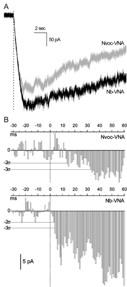
FIGURE 5: Comparison of inward currents activated by photorelease of Nb-VNA and Nvoc-VNA in nodose ganglion neurons. (A) Whole-cell currents recorded in rat nodose ganglion neurons loaded with Nb-VNA (black trace; average of 3 experiments) or Nvoc-VNA (gray trace; average of 2 experiments), and voltage-clamped at -55 mV. Cells were loaded by incubation with 5 \mu\text{M} caged vanilloid for \sim 7 min and then superfused with physiological saline. Currents were activated by a 5-ms flash of 355-nm light delivered to a 10\text{-}\mu\text{m} spot positioned over the edge of the neuron (typically 35\text{--}50 \mu\text{m} in diameter). Photolysis was thus restricted to a small region near the plasma membrane. The dashed line marks the start of the photolytic flash. The UV exposure was 1.1 \mu\text{J}/\mu\text{m}^2 . (B) Time courses of whole-cell currents around the time of photolysis shown at higher resolution. Data from Figure 5A were grouped into 1-ms intervals, and the average current in each interval was plotted as a bar graph against time (upper panel, Nvoc-VNA data; lower panel, Nb-VNA data); vertical dotted lines mark the start of the 5-ms flash. Current levels corresponding to 2 and 3 standard deviations ( 2\sigma and 3\sigma ) from baseline are marked by thin horizontal lines in each panel. The current activated by Nvoc-VNA exceeded the 2\sigma level after 13 ms, and the 3\sigma level after 32 ms. The current activated by Nb-VNA exceeded both the 2\sigma and 3\sigma levels in <4 ms.
