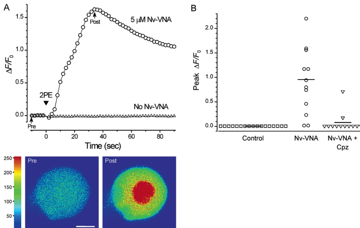
FIGURE 6: Effect of 2-photon photolysis of Nv-VNA on nodose ganglion neurons. (A) In situ 2-photon photolysis of Nv-VNA evokes robust [Ca^{2+}]_i rises in nodose ganglion neurons. Fluorescence traces acquired in two separate experiments from single nodose ganglion neurons that had been loaded with the fluorescent Ca^{2+} indicator, fluo-3. When the neuron was superfused for 5 min with Locke solution containing 5 \mu M Nv-VNA, scanning 2-photon excitation (arrowhead marked "2PE") evoked a sharp rise in [Ca^{2+}]_i (circles), as reflected by a large increase in fluo-3 fluorescence. In contrast, in a neuron not incubated with Nv-VNA, 2-photon excitation evoked no response (triangles). During 2-photon excitation, the Ti:S laser beam was scanned across the cell 10 times; each pixel ( 0.22 \times 0.22 \mu\text{m}^2 ) received 16 \mu\text{s} of total exposure, corresponding to total exposure of \sim 100 nJ per pixel, or \sim 2 \mu\text{J}/\mu\text{m}^2 . Representative pre- and postphotolysis confocal fluorescence images of the responsive neuron, corresponding to points in the trace marked by arrows, are shown below the graph. Fluorescence intensity in the images is encoded in pseudocolor. Scale bar = 10 \mu\text{m} . (B) The [Ca^{2+}]_i rise in nodose ganglion neurons evoked by 2-photon photolysis of Nv-VNA is blocked by capsazepine, a vanilloid receptor antagonist. None of 17 control neurons exposed to the pulsed 720-nm emission from a titanium-sapphire laser in the absence of Nv-VNA showed a [Ca^{2+}]_i response. In the presence of 5 \mu M Nv-VNA, the same exposure to 720-nm light evoked [Ca^{2+}]_i rises in 12 of 14 neurons. In the presence of 5 \mu M Nv-VNA and 5 \mu M capsazepine (Cpz, a vanilloid antagonist), the same exposure to 720-nm light triggered a significant response in only 1 out of 11 neurons. Solid horizontal lines indicate the mean peak \Delta F/F_0 for each population: control, 0.003 \pm 0.0008 ( n = 17 ); in the presence of Nv-VNA, 0.96 \pm 0.17 ( n = 14 ); in the presence of Nv-VNA and Cpz, 0.078 \pm 0.0593 ( n = 12 ).
